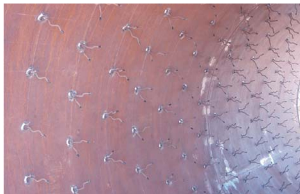
Essar Refinery Project Monolithic Refractory Lining.
